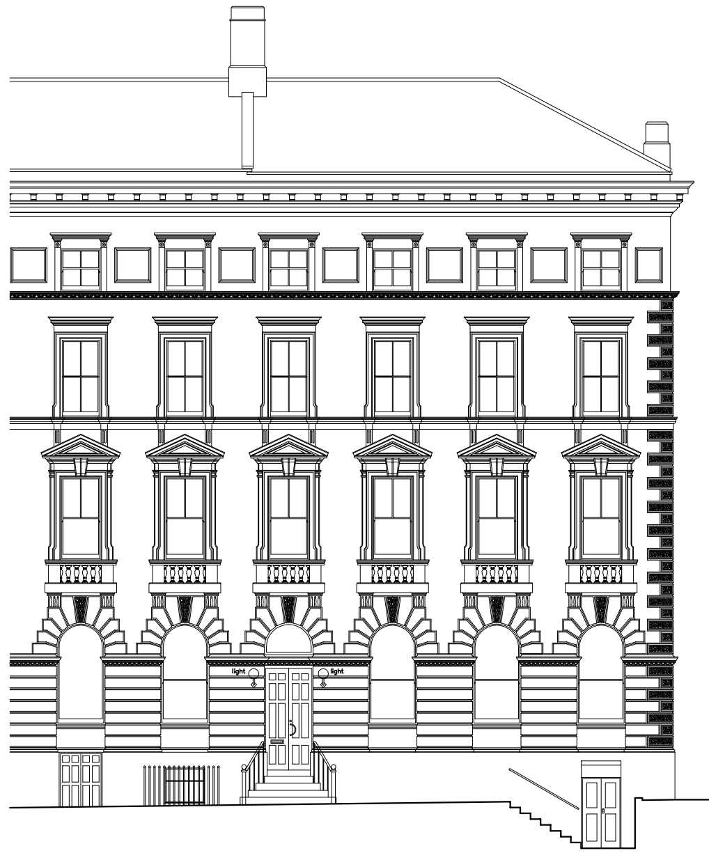
FRONT ELEVATION (ST GEORGES SQUARE)
